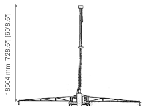
UP VIEW
