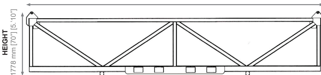
SIDE VIEW 7925 mm [312"] [26']
