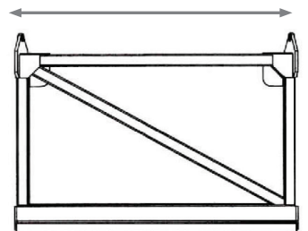
FRONT VIEW 2438 mm [96"] [8']
