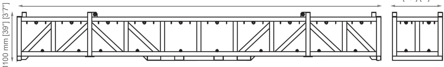
FRONT VIEW 1200 mm [48"] [4']
