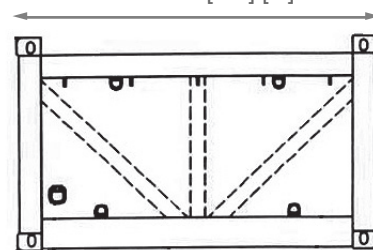
FRONT VIEW 2438 mm [96"] [8']
