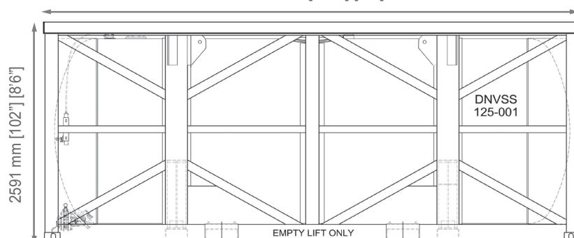
SIDE VIEW 6058 mm [238"] [20']
