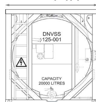
FRONT VIEW 2438 mm [96"] [8']
