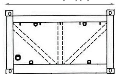
FRONT VIEW 2438 mm [96"] [8']
