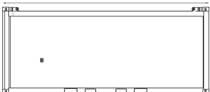
SIDE VIEW 6058 mm [240"] [20']
