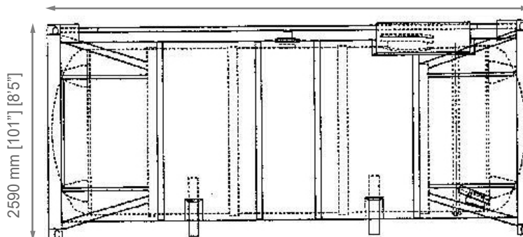
SIDE VIEW 6096 mm [240"] [20']
