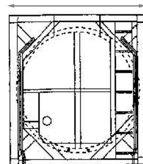
FRONT VIEW 2438 mm [96"] [8']
