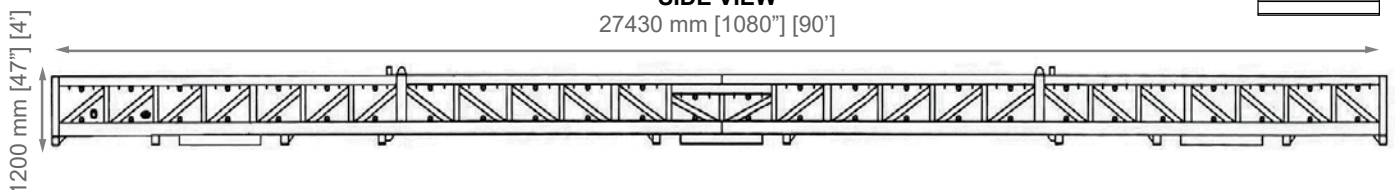
SIDE VIEW
